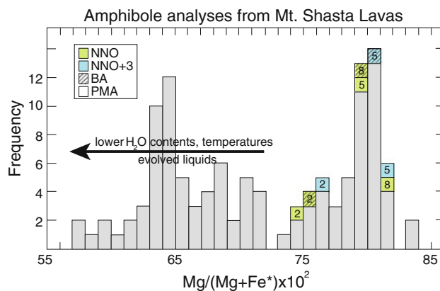
Fig. 10 Histogram of amphibole phenocryst Mg#s from Mt. Shasta lavas from Grove et al. (2005). Also plotted are the experimental amphiboles we have produced in this study. Each experimental amphibole is labeled with its pressure in kbar, and the estimated \text{H}_2\text{O} content necessary to precipitate it. Experimental amphiboles range in f_{\text{O}_2} , and are both primitive magnesian andesite and BA. The high-Mg# peak in the Mt. Shasta region amphiboles is proposed to represent deep and \text{H}_2\text{O} -rich fractionation
