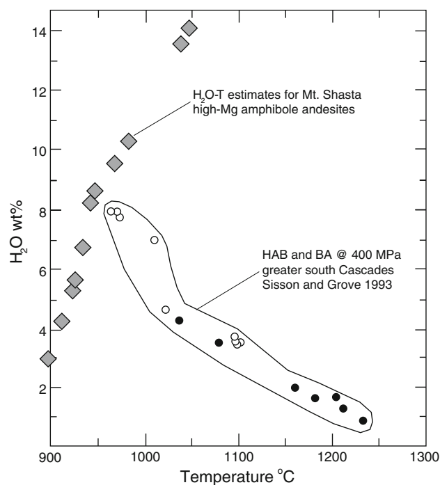
Fig. 11 Dissolved H 2 O content and magmatic temperatures are estimated for the parental magmas crystallizing high-Mg# amphiboles in Mt. Shasta lavas modified after Grove et al (2012). Experimental amphibole Mg# and temperatures were used to make a calibration curve to determine the temperature of parental magma to the Shasta amphiboles in Table 5. Pressure estimates come from the amphibole Mg# barometer calibrated for these specific magmas. Pressure estimates were then converted to H 2 O contents assuming water saturation and using a mixture of 75 % basalt and 25 % rhyolite solubilities at 1,000 °C from VolatileCalc. The trend defined by the Mt. Shasta samples ( diamonds ) defines an H 2 O-saturated crystallization trend of magmas as they ascend through the crust, so the high-H 2 O, high T samples are the deepest and the low H 2 O and low T are the shallowest. The HAB and BA trend of S. Cascades lavas is from Sisson and Grove (1993) and represents variable melting processes that produce variable water contents for mantle derived melts
