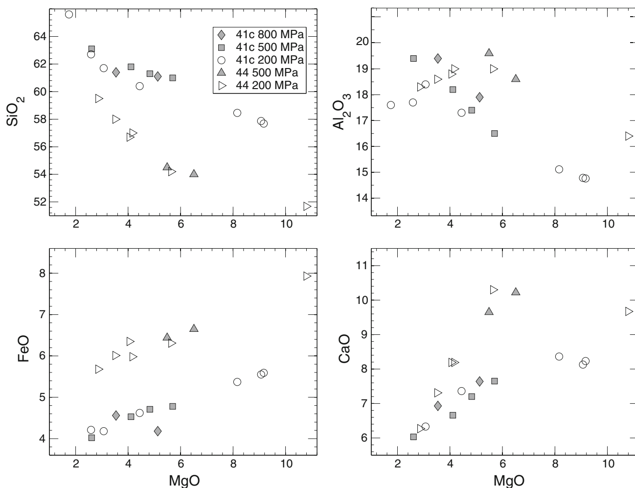
Fig. 5 Variation diagrams showing the compositions of experimental glasses, with the composition normalized anhydrous. Crystallization over a wide range of pressure produces indistinguishable compositions
