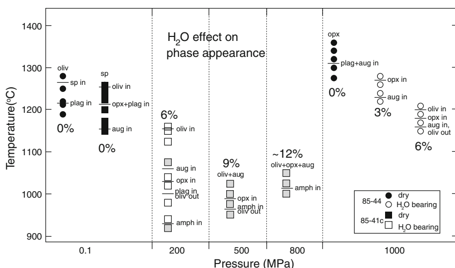
Fig. 7 Experimental crystallization sequences for the primitive magnesian andesite water-saturated compared to the experiments of Baker et al. (1994) on the basaltic andesite at various \text{H}_2\text{O} contents. Note the very large temperature difference and different phase assemblages in the basaltic andesite and primitive magnesian andesite at high pressure and varying \text{H}_2\text{O} content. Both magmas have very
