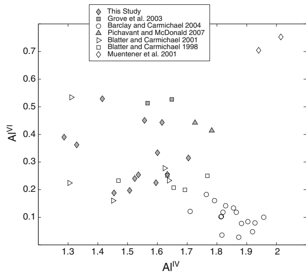
Fig. 4 Calculated Al site partitioning in experimental amphiboles crystallized from primitive arc magma starting materials from this study and the experimental literature. For these high thermodynamic variance systems there is no observable trend with tetrahedrally coordinated Al vs. octahedrally coordinated Al. Site assignments are calculated with the algorithm of Leake et al. (1997) on a 23 oxygen basis
