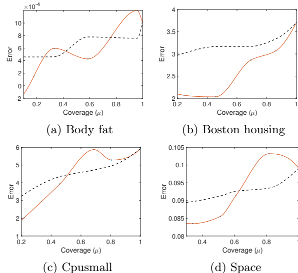
Figure 1: RC curves of Algorithm 1 (red line) and the baseline method (dashed line) on different regression data sets from the LIBSVM repository. The horizontal axis represents the coverage ( \mu ), while the vertical axis represents the error.
