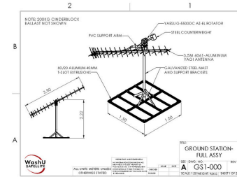
Engineering Drawing of GS-1
