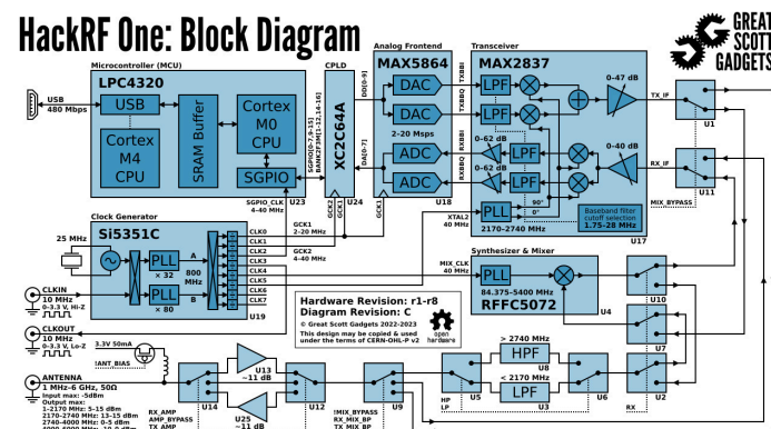
Block Diagram of GS-1 SDR
