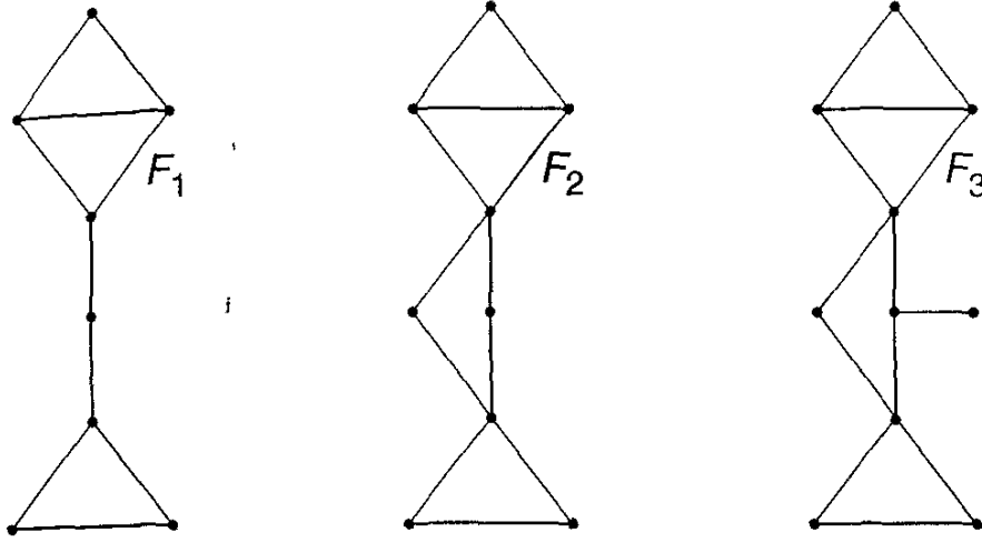
Fig. 4.1. F_1 is balanced, F_2 is strictly balanced and F_3 is not balanced.
