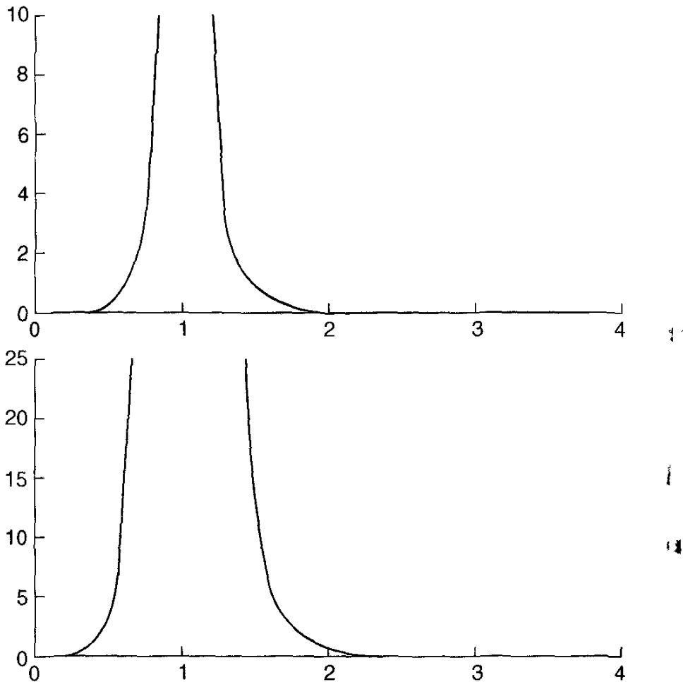
Fig. 5.5. The curves of E_{c/n}(X) and \sigma^2_{c/n}(X) .
