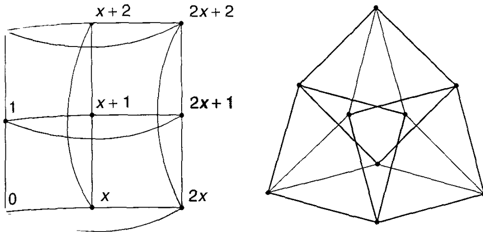
Fig. 13.1. Two drawings of the Paley graph P_9 , with \mathbb{F}_9 = \mathbb{Z}_3[x]/(x^2 + 1) .
