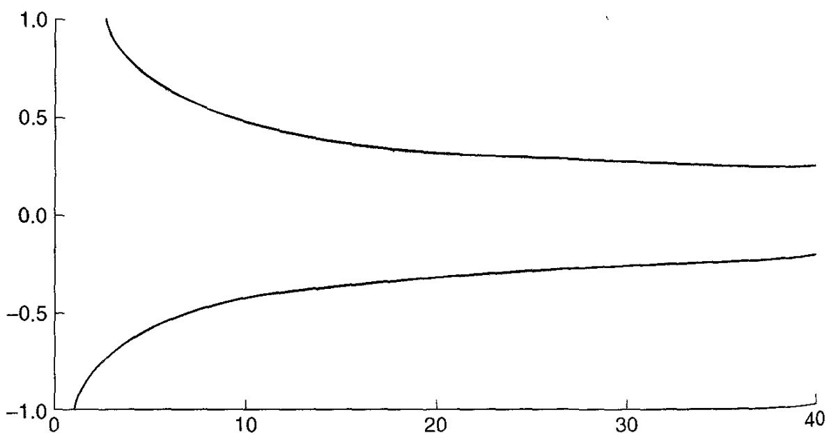
Fig. 3.1. The functions \eta_\Delta(c) and \eta_\delta(c) .
