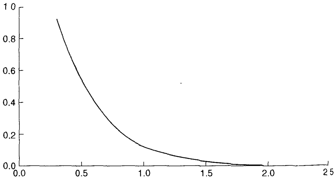
Fig. 5.3. The function \mu(c) = (1/6\sqrt{3\pi}) \int_{c^3/6}^\infty v^{-3/2} e^{-v} dv , the limit of the expected number of isolated trees of order at least cn^{2/3} in G_{1/n} .
