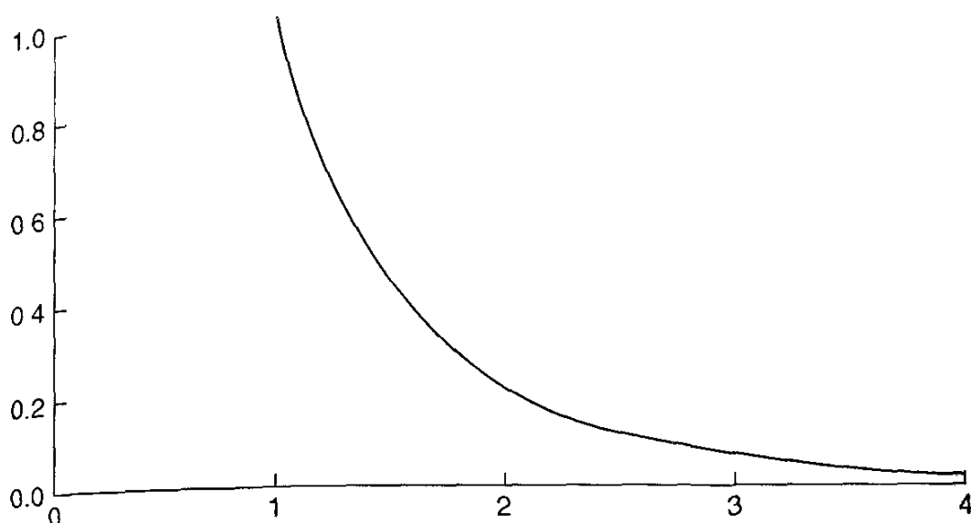
Fig. 5.1. The curve y = t(c) .
