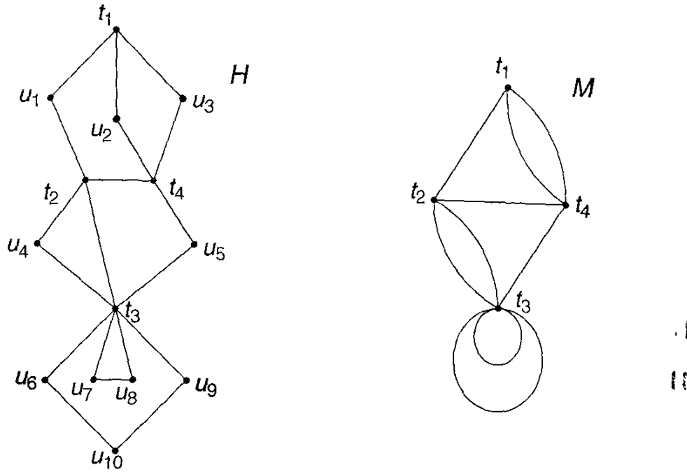
Fig. 5.4. A graph H and a multigraph M with T = \{t_1, \dots, t_4\} and U = \{u_1, \dots, u_{10}\} .
