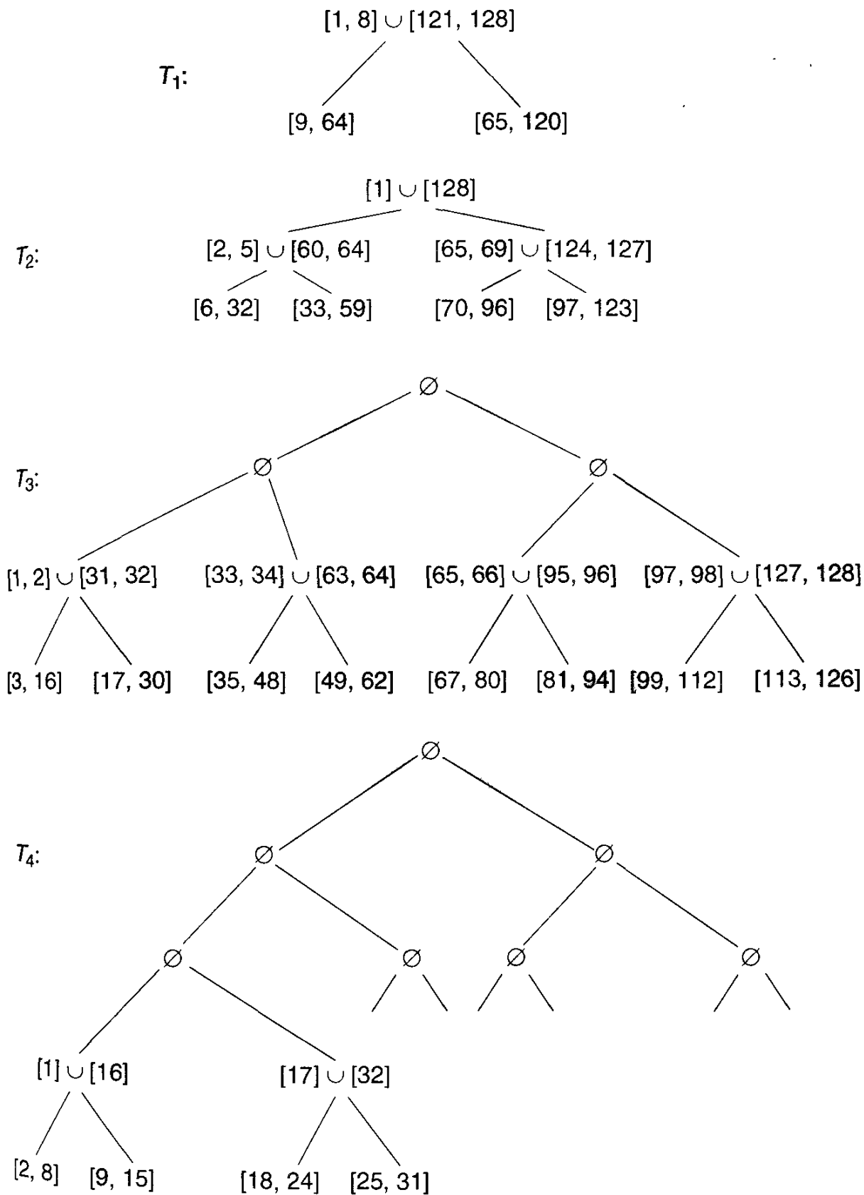
Fig. 15.1. The partitions of [1, 128] corresponding to T_1 , T_2 , T_3 and T_4 for A = 4 .
