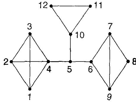
Fig. 4.2. A graph F with m(F) = 3 and d(F) = 17/6 .
