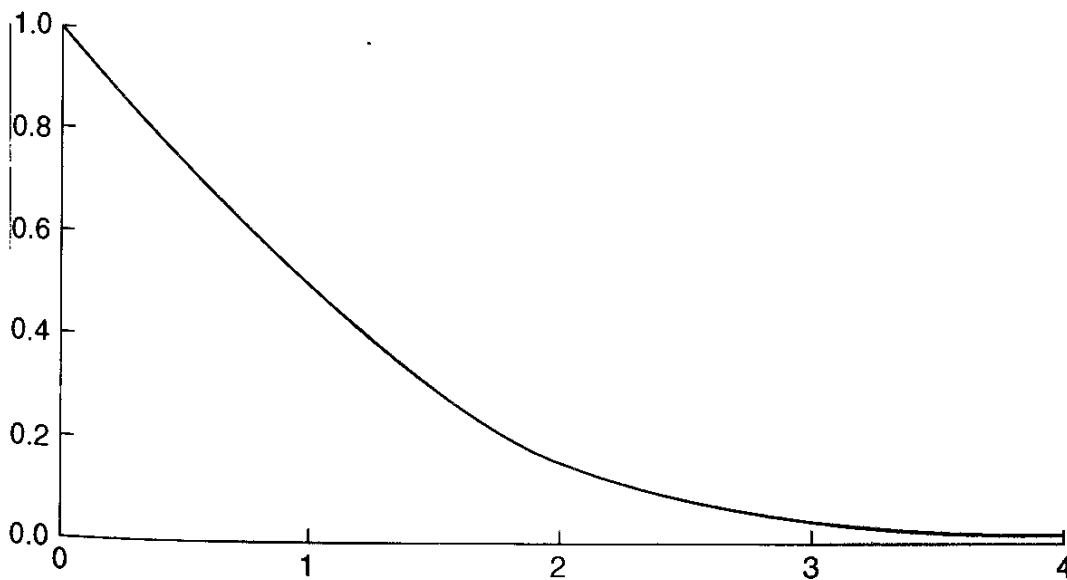
Fig. 5.2. The function u(c) .
