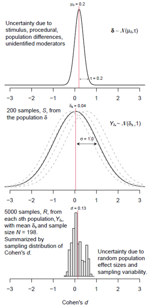
Figure 6. Illustration of the simulation of random population effect sizes and sampling variability. Uncertainty in the population effect size ( \tau ) is combined with sampling variability (samples drawn from S populations) and summarized in the sampling distribution of Cohen's d .
