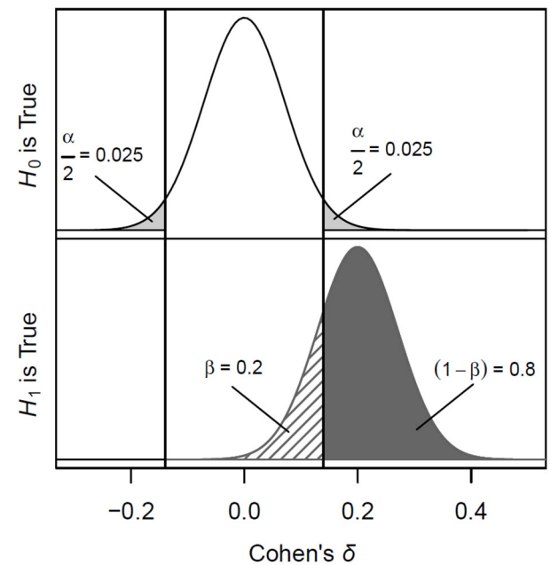
Figure 1. Power = .8 as area under the sampling distribution of H_1: \delta = 0.2 , with H_0: \delta = 0 , when N = 198 and \alpha = .05 for a two-sided dependent samples t -test (see also Condition D in Figure 2).
