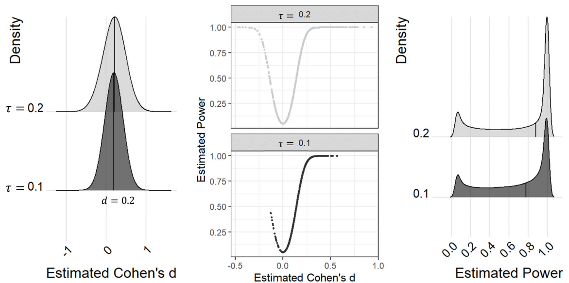
Figure 7. The joint effect of random population effect sizes and sampling variability of estimated d in the calculation of power. The left panel illustrates the sampling variability in estimated d when \mu_d = 0.2 , N = 198 (cf. point D of Figure 2), and \tau = 0.1 or 0.2 . The middle panel presents calculated power values in relation to the estimated effect size d . The right panel presents the density plot of power values, ignoring the direction (sign) of the estimated effect d (visible in the middle panels).
