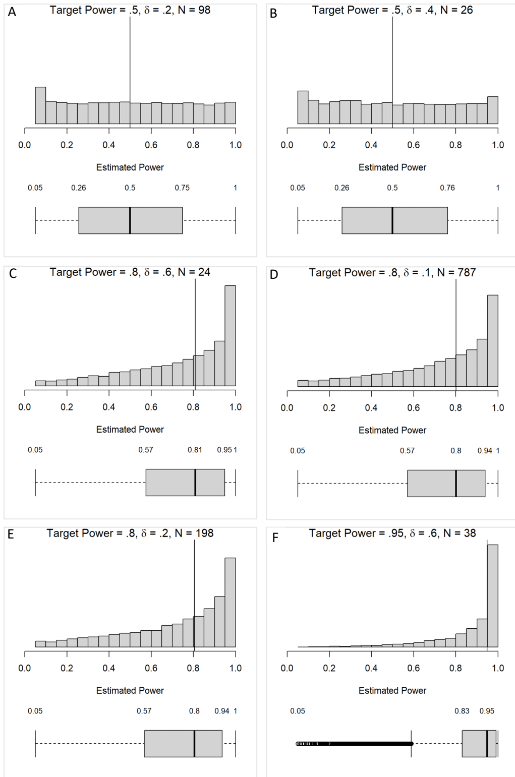
Figure 4. Histograms and boxplots of power estimates for a two-sided t -test from a two-condition within-subjects design that reflect uncertainty due to the sampling variability in the effect size estimate ( d ) for six simulated conditions (see Figure 2). Within each panel, the title denotes the population effect size value, \delta , and sample size ( N ) that obtains target power calculated via the classical approach.
