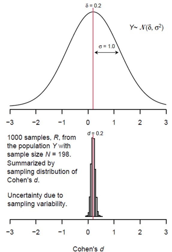
Figure 3. Illustration of the simulation showing sampling variability in the estimated effect size. Population distribution with mean \delta = 0.2 and standard deviation \sigma = 1 (point D in Figure 2), and sampling distribution of Cohen's d for 1000 samples.
