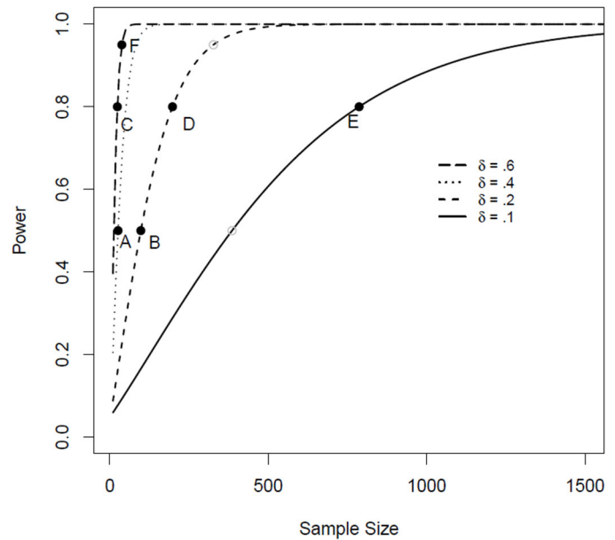
Figure 2. The nonlinear relationship between sample size ( N ), effect size ( \delta ), and power for a two-condition within-subjects design for a two-sided t -test where \alpha = .05 . Points labeled A to F relate to the six conditions (unique combinations of N , \delta , and power) in the simulation. Condition D is depicted in Figure 1.
