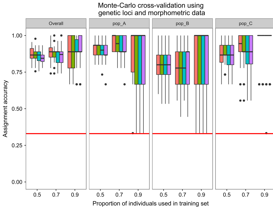
FIGURE 4 Assignment accuracies estimated via Monte-Carlo cross-validation and support vector machine methods, with random sampling of three levels of training individuals crossed by four levels of training loci (each box cluster from left to right: 10%, 25%, 50%, all) plus four morphometric measurements crossed by 30 iterations. See Figure 2 for box plot description details
