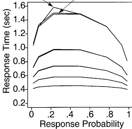
Figure 7. An illustration of what happens to the fit of the diffusion model if one error quantile is increased (cf. the change in one data point in Figure 4).
