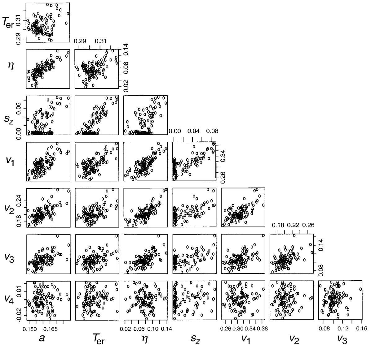
Figure 6. Scatterplots among the parameters of the diffusion model for fits to simulated data, using the maximum likelihood method (using parameters from line 3 in Table 1).
