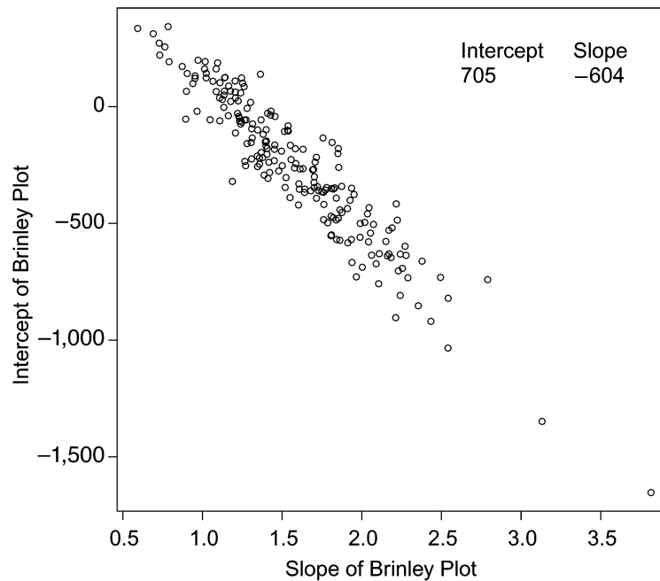
Figure 1. A plot of intercept and slopes from Brinley functions when there is random variation across 200 simulated experiments in the overall means and SDs across conditions. For each simulated experiment, for older subjects, a mean RT was selected from a normal distribution with mean 700 msec and SD 70 msec, and an SD was selected from a normal distribution with mean 150 msec and SD 30 msec. For young subjects, a mean RT was selected from a normal distribution with mean 600 msec and SD 50 msec, and an SD was selected from a normal distribution with mean 100 msec and SD 20 msec. The Brinley slope and intercept were calculated for each of the 200 simulated experiments, and these provide the basis of the plot.
