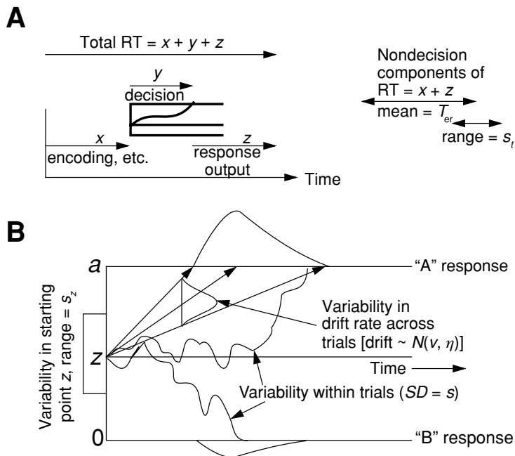
Figure 1. An illustration of the diffusion model. Parameters of the model are a = boundary separation (one value, a_{sp} , for speed instructions and another, a_{ac} , for accuracy instructions); z = starting point; T_{er} = mean time for nondecision components of RT; \eta = SD in drift across trials; s_z = range of the distribution of starting points across trials; v = drift rate (one for each level of difficulty in an experiment); s_t = range of the distribution of nondecision times across trials; s = SD of variability in drift within trials. s is a scaling parameter, set to 0.1 as in previously published fits of the model.
