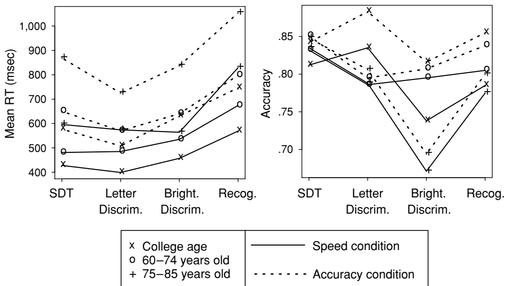
Figure 2. Mean values of correct RT and accuracy, averaged across subjects and experimental conditions for each task and each group of subjects. For both mean RTs and accuracy, the top line of the pair of lines for a group in each panel is for conditions with accuracy instructions, and the bottom line is for conditions with speed instructions.
