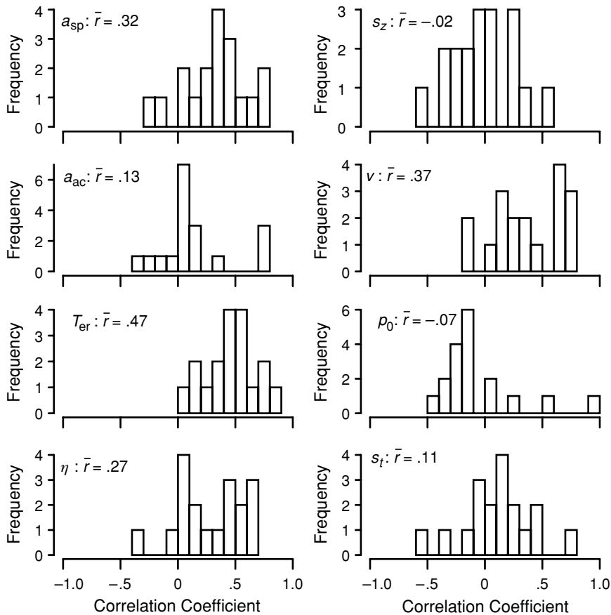
Figure 4. Histograms of correlations for parameter values of the model across all pairs of the four experiments and across the three subject groups. The mean values of the correlations are shown, and the critical value of the mean correlation is .14. p_0 is the proportion of contaminants estimated using the method of Ratcliff and Tuerlinckx (2002).
