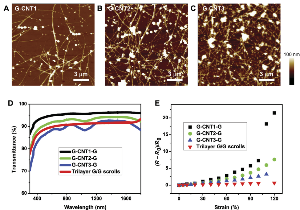
Fig. 3. Exploration of CNTs as a replacement of graphene scrolls. (A to C) AFM images of three different densities of CNTs (CNT1<CNT2<CNT3) on graphene. (D) Optical transmittances of G-CNT-G on quartz. (E) Normalized resistance change of G-CNT-G as a function of strain. Transmittance and normalized resistance change of trilayer MGGs are listed as a comparison.
