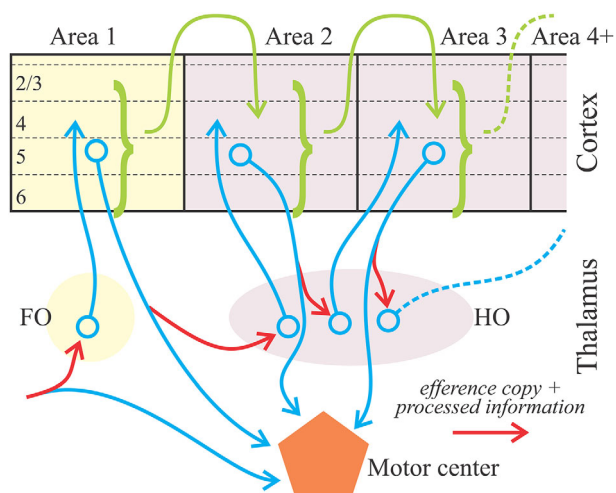
FIGURE 1 Schematic showing aspects of thalamocortical relationships involving feedforward circuits ascending a hierarchy. Cortical areas are connected both by direct pathways (green arrows) and transthalamic ones involving higher-order (HO) thalamic nuclei. Note that the inputs to both first-order (FO) and higher-order thalamic relays arrive via branching axons (blue and red arrows), with extrathalamic branches innervating a motor center (blue arrows), and the branch innervating thalamus (red arrows) carrying a message that can be interpreted as an efference copy as well as other processed information
