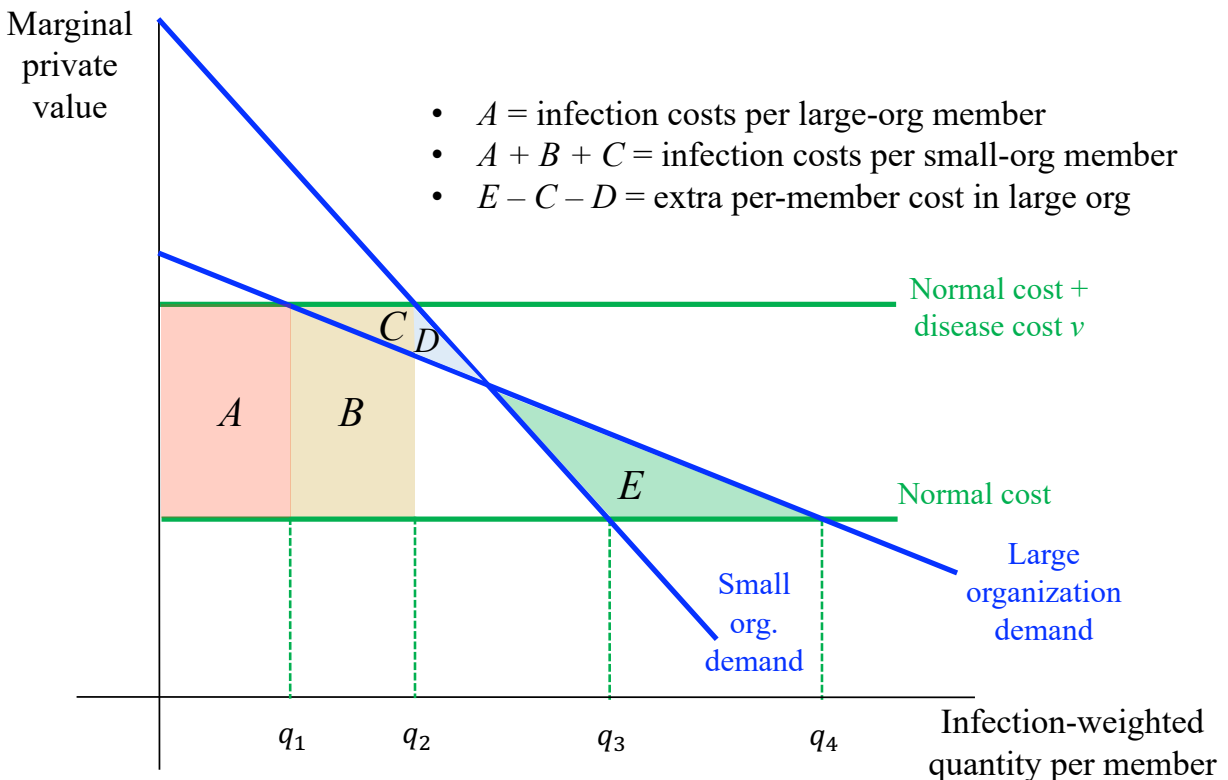
Figure A1. Infections and Prevention for Small and Large Organizations
