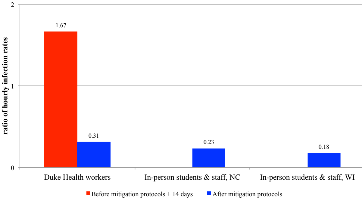
Figure 3. COVID-19 Infections Acquired at Work or School as a Ratio to those Acquired in the Community
