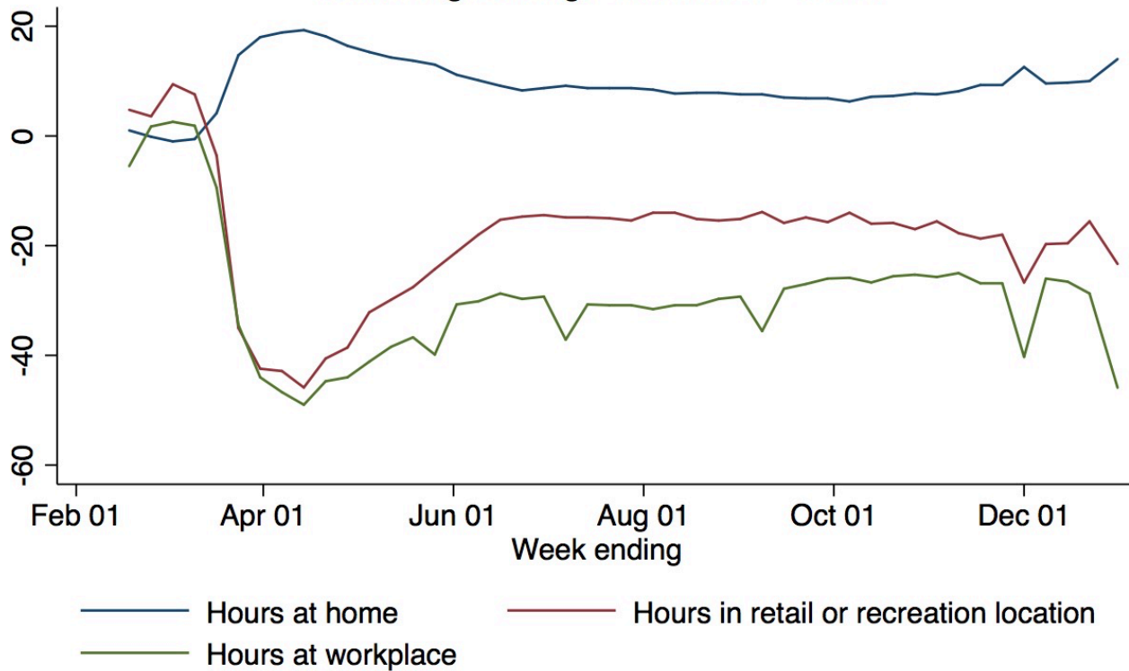
Figure 2. U.S. Weekly Mobility, 2020 Percentage change from Jan 3 - Feb 6
