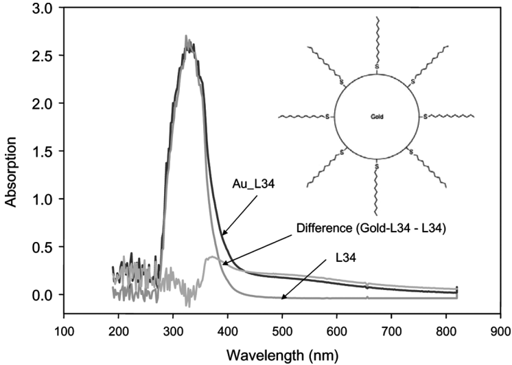
FIGURE 2 Schematic depiction of the dodecanethiol – coated gold nanoparticles and the resulting absorption spectra of L34 and the Au-Nano doped L34 and the. Bottom right curve shows the differential absorption spectrum of dodecanethiol – coated gold.
