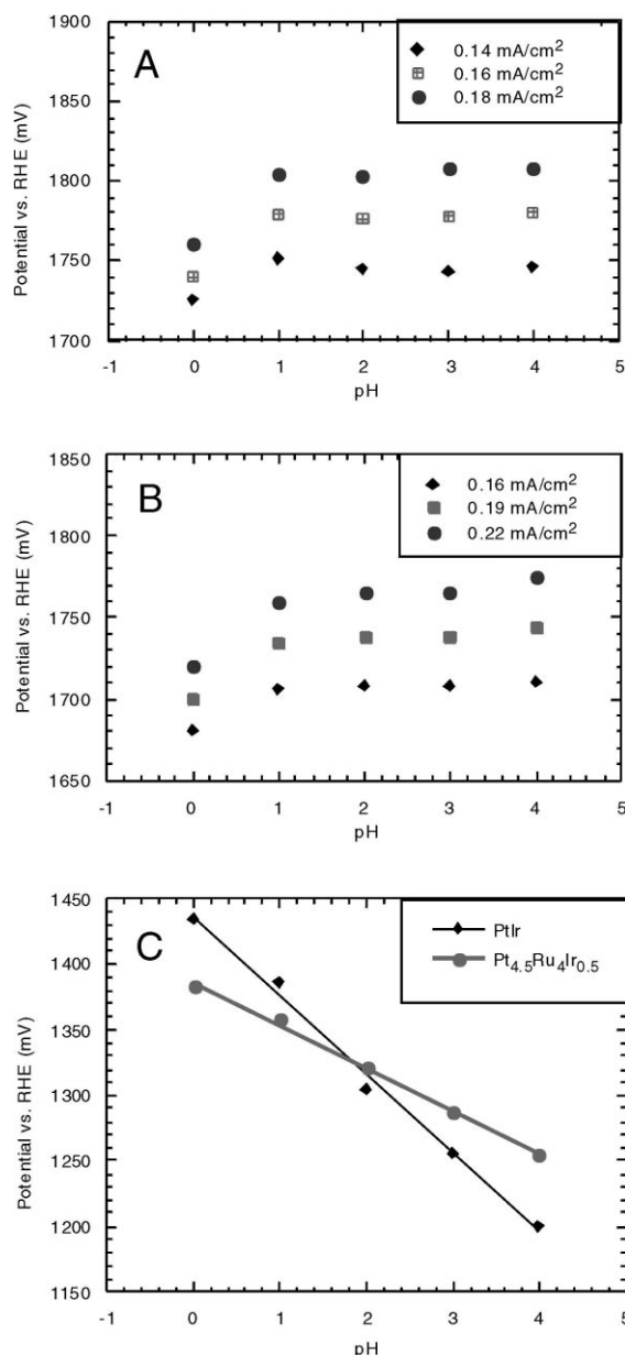
Fig. 7. pH dependence of electrode potential for: (A) Pt 4.5 Ru 4 Ir 0.5 at high current density; (B) PtIr at high current density; (C) Pt 4.5 Ru 4 Ir 0.5 and PtIr at low current density ( 2 \times 10^{-3} mA/cm 2 ).
