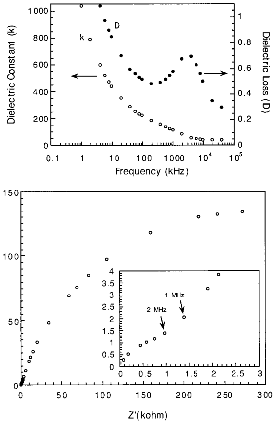
Figure 7. Frequency dependence of the dielectric constant and loss for HCa_2Nb_3O_{10} at 70 °C (top), and complex impedance plot (bottom) for HCa_2Nb_3O_{10} . The inset plot (bottom) of -Z'' vs Z' at high frequency shows partial resolution of a low-impedance semicircle.
