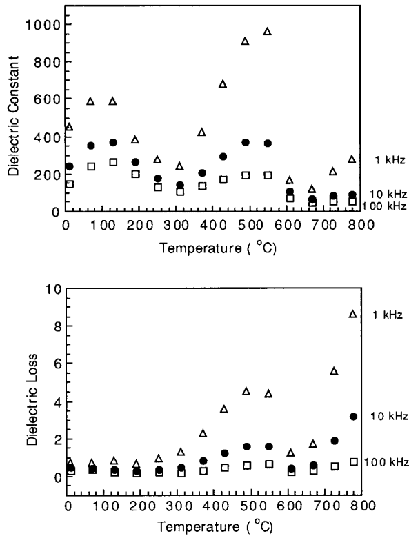
Figure 6. Dielectric constant (top) and loss (bottom) of HCa_2Nb_3O_{10} at 1, 10, and 100 kHz, as it is heated and transformed first to Ca_4Nb_6O_{19} , and then to a mixture of CaNb_2O_6 and Ca_2Nb_2O_7 .
