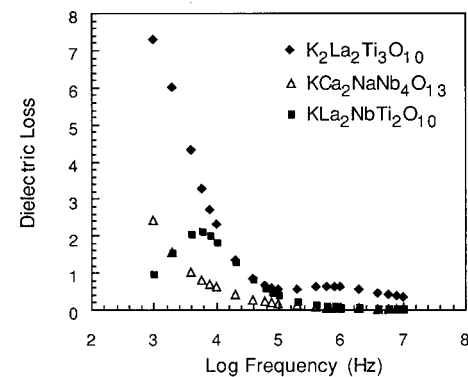
Figure 10. Dielectric constant (top) and loss (bottom) vs frequency for the Ruddlesden–Popper compound \text{K}_2\text{La}_2\text{Ti}_3\text{O}_{10} , and for Dion–Jacobson compounds \text{KCa}_2\text{NaNb}_4\text{O}_{13} and \text{KLa}_2\text{NbTi}_2\text{O}_{10} .
