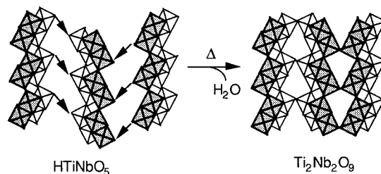
Figure 1. Schematic structural representation of the topochemical condensation of HTiNbO 5 to Ti 2 Nb 2 O 9 , reaction 1 (data from ref 11).
