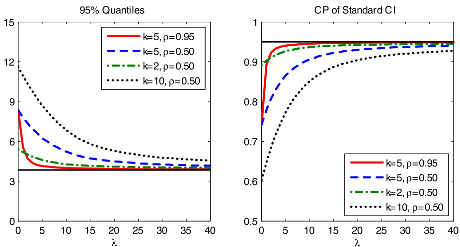
FIGURE S-32.—Asymptotic 95% quantiles of the QLR statistic and asymptotic coverage probabilities of standard CI's concerning the structural parameter \pi in the linear IV model.
