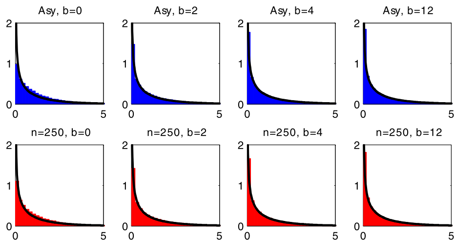
FIGURE S-18.—Asymptotic and finite-sample ( n = 250 ) densities of the QLR statistic for the AR parameter \rho in the ARMA(1, 1) model when \rho_0 = 0.4 and the \chi^2_1 density (black line).
