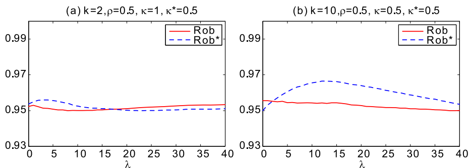
FIGURE S-30.—Coverage probabilities of robust QLR CI's for the structural parameter \pi in the linear IV model, k = 2, 10 , \rho = 0.5 . The ICS statistics for Rob and Rob* are the null-imposed and unrestricted Wald statistics.
