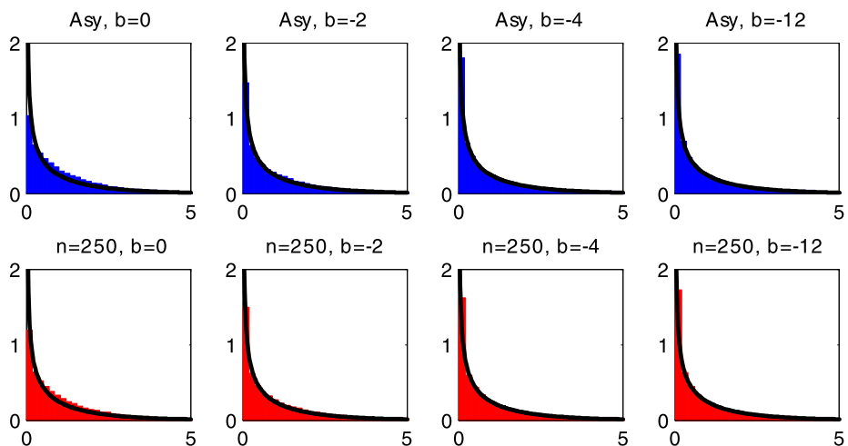
FIGURE S-5.—Asymptotic and finite-sample ( n = 250 ) densities of the QLR statistic for the MA parameter \pi in the ARMA(1, 1) model when \pi_0 = 0 and the \chi^2_1 density (black line).
