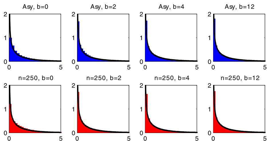
FIGURE S-19.—Asymptotic and finite-sample ( n = 250 ) densities of the QLR statistic for the AR parameter \rho in the ARMA(1, 1) model when \rho_0 = 0.8 and the \chi^2_1 density (black line).
