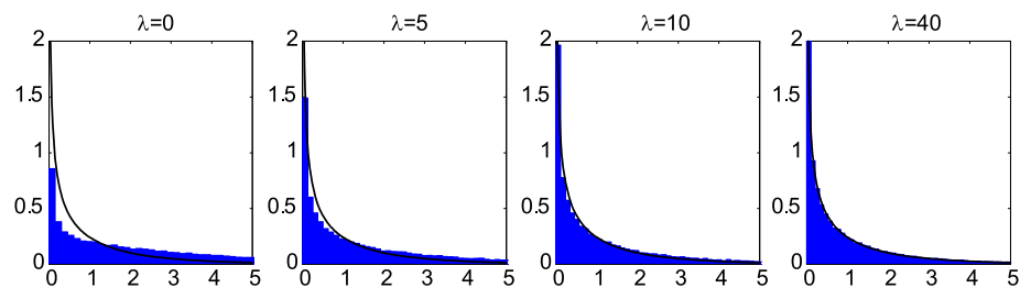
FIGURE S-31.—Asymptotic densities of the QLR statistic for the structural parameter \pi in the linear IV model when k = 5 , \rho = 0.5 and the \chi^2_1 density (black line).
