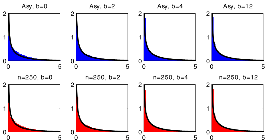
FIGURE S-17.—Asymptotic and finite-sample ( n = 250 ) densities of the QLR statistic for the AR parameter \rho in the ARMA(1, 1) model when \rho_0 = 0 and the \chi^2_1 density (black line).
