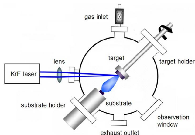
Figure 3. Experimental setup for graphene growth using Pulsed Laser Deposition. Adapted from [49]. Copyright IOP Science 2014.
