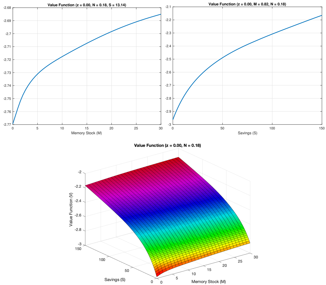
Figure 6: Value Function
