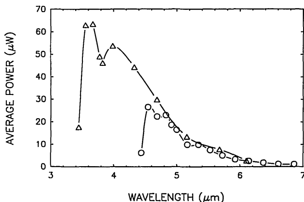
Fig. 2. Average IR output power as a function of IR wavelength. The curve from 3.4 to 6.2 \mu\text{m} was taken by using LDS 821 dye, and the curve from 4.4 to 7.0 \mu\text{m} was taken by using LDS 867 dye. Note that by using a different output coupler it is possible to extend the tuning range as far as 9.14 \mu\text{m} to the red (see text).
