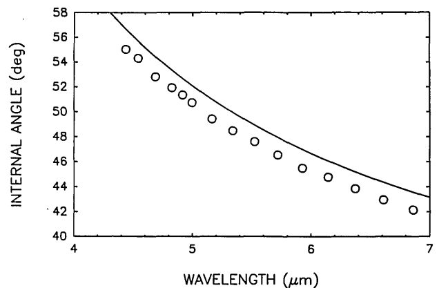
Fig. 3. Variation of \text{AgGaS}_2 phase-matching angle with respect to IR wavelength. Experimental data are represented by open circles. The solid curve is obtained theoretically with the Sellmeier equation 18 and index of refraction data from Ref. 12.
