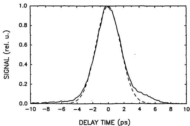
Fig. 5. Cross-correlation between IR output pulse at 5 \mu\text{m} and the frequency-doubled compressed YAG pulse ( \lambda = 0.532 \mu\text{m} ). The dashed curve represents the best Gaussian fit to the pulse shape.
