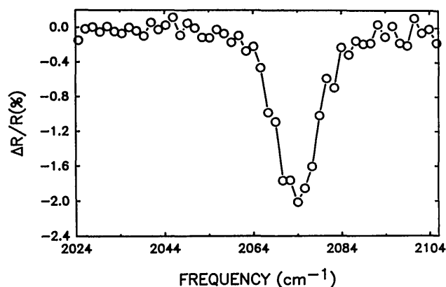
Fig. 6. Results of a single 1-min linear absorption scan that uses the source to probe the atop resonance of CO adsorbed on Cu[111] at 110 K in ultrahigh vacuum.
