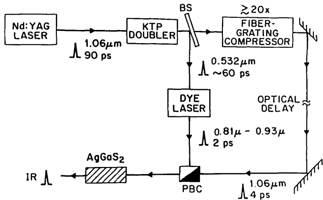
Fig. 1. Schematic of the laser system used to generate IR. BS represents a dichroic beam splitter, and PBC represents a polarizing beam combiner.
