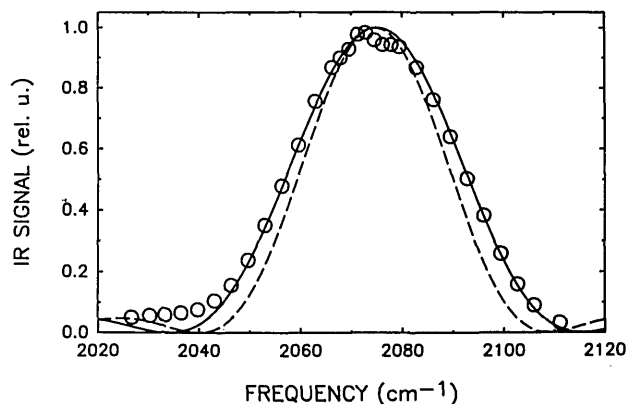
Fig. 4. IR average power as a function of wavelength for a fixed crystal orientation. Experimental data are open circles. Solid (dashed) curve is a fit to theory for an interaction length of 1.6 mm (1.4 mm).
