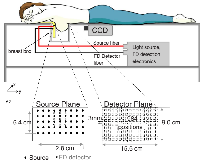
Fig. 1 Schematic of the parallel plate diffuse optical tomography instrument. A female subject lies in prone position on a bed with her breasts inside the breast box filled with an Intralid/Ink fluid. Continuous-wave transmission and frequency-domain remission measurements are performed simultaneously by a CCD camera and nine Avalanche Photodiodes connected by fibers on the source plate for 45 source positions at multiple wavelengths.
