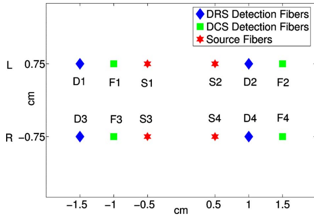
Fig. 1 Arrangement of the optical probe. Four multimode source fibers ( \star ), four 1-mm DRS fibers ( \blacklozenge ), and four single-mode DCS fibers ( \blacksquare ) were used for simultaneous DRS and DCS measurements. The fibers were arranged into two columns, oriented anteriorly posteriorly along most of the length of the left and right cerebral hemispheres on top of the piglet head. The source-detector separations ranged from 5 mm to 2 cm.
