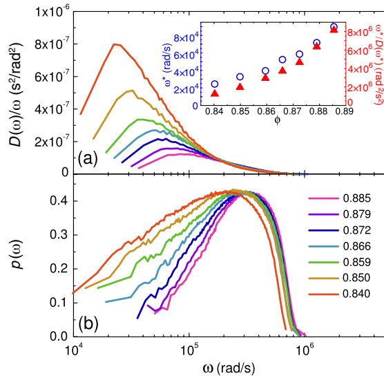
FIG. 4 (color online). (a) D(\omega)/\omega and (b) participation ratio vs \omega as a function of packing fraction [as labeled in (b)]. Inset to (a): the boson peak frequency \omega_b (circles, left) and inverse peak height \omega_b/D(\omega_b) (triangles, right) vs \phi .
