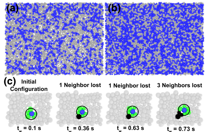
FIG. 3 (color online). Particle configuration snapshots. (a) Snapshot of colloidal glass immediately after the quench, at t_w = 0.03 s. Particles with six nearest neighbors are plotted in blue. (b) Snapshot of aged colloidal glass long after the quench, at t_w = 10,000 s. Particles with six nearest neighbors are plotted in blue. (c) Example of an irreversible rearrangement that finishes at t_w = 0.67 s. The irreversibly rearranging particle is blue, its nearest neighbors are green, and nearest neighbors it loses are black. The circle represents the cutoff distance that defines nearest neighbors.
