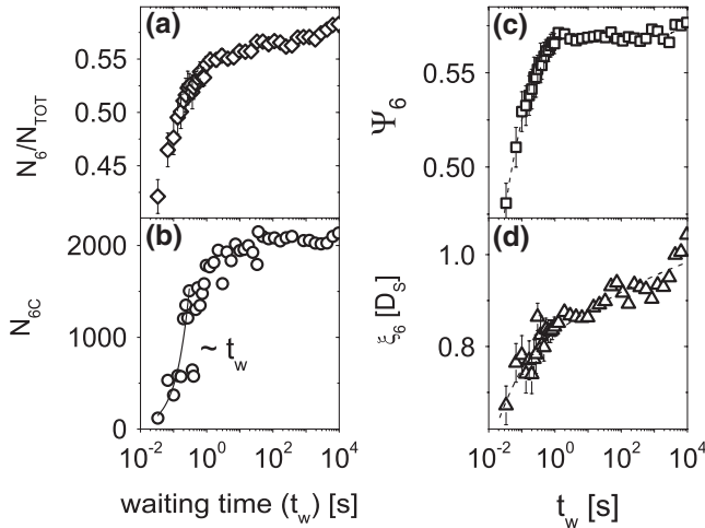
FIG. 4. Growth of local order during aging. (a) N_6/N_{\text{tot}} , the fraction of particles with a coordination number of 6 versus t_w . (b) N_{6C} , the number of particles in the largest cluster of particles with 6 nearest neighbors versus t_w . (c) Bond orientational order parameter, \psi_6 versus t_w . (d) Orientational order correlation decay length \xi_6 , extracted from g_6 , versus t_w .
