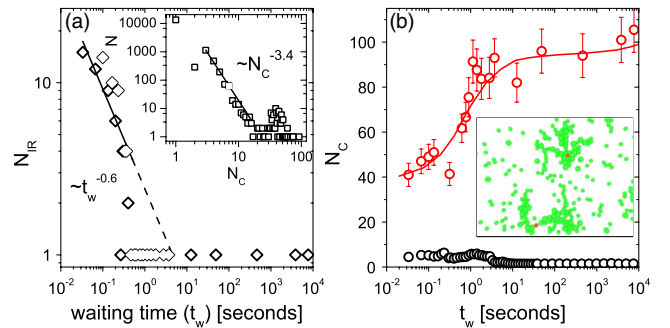
FIG. 2 (color online). Irreversible rearrangements during aging. (a) N_{\text{IR}} , the number of irreversible rearrangements, versus t_w . The line is a power law fit to guide the eye. Inset: Histogram of N_C , fast particle cluster sizes, for 0.03 \leq t_w \leq 3 sec. The line is a power law fit to guide the eye. (b) Average number of fast particles per cluster for all clusters (black circles) and the average number of fast particles per cluster for only clusters containing a particle undergoing an irreversible rearrangement (red circles), versus t_w . The line guides the eye. Inset: Snapshot of the 10% fastest particles at t_w = 0.62 sec, featuring two large clusters. Particles that irreversibly rearrange are plotted in red.
