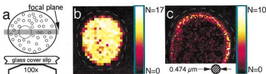
FIG. 1. (a) Cartoon of the 600-nm-thick slice through an SOPC vesicle imaged with an optical microscope. We measured the in-plane positions of the larger colloidal sphere when it was in focus. (b) (color) Probability distribution of a single 0.237- \mu\text{m} -radius polystyrene sphere inside a vesicle (no small spheres). The white dashed line is the edge of the vesicle, and the colored points indicate the number of times, N , the center of the sphere was observed in a bin located at a given point. There were 2000 events and the bins were 130 \times 130 nm. The sphere simply diffused freely throughout all of the available space. (c) (color) Same as in (b), but with a vesicle that also contained small spheres ( \phi_S = 0.30 , R_S = 0.042 \mu\text{m} , \alpha = 5.7 ). There were 2300 events and the bin size was 65 nm. The large sphere was clearly attracted to the vesicle wall, especially where the vesicle was most curved.
