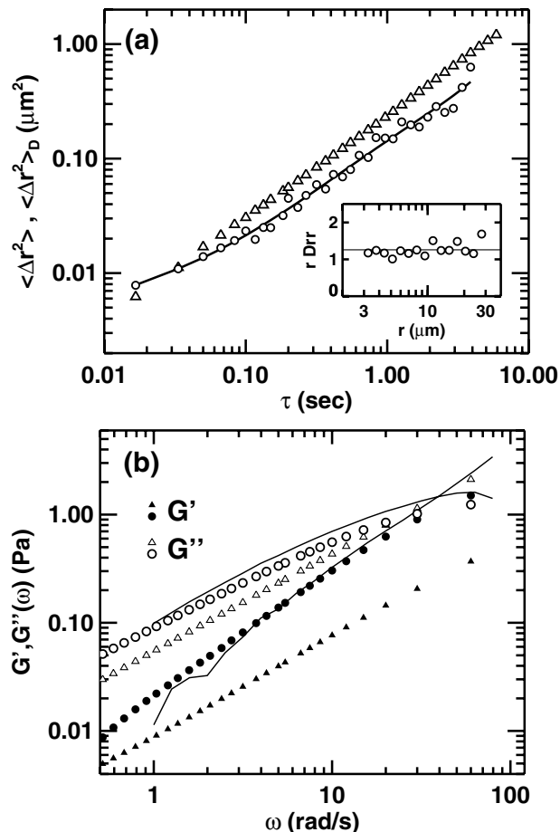
FIG. 2. (a) Comparison of the self (triangles) and distinct (circles) displacements of 0.20 \mu\text{m} diameter beads in 0.25% weight guar solution. The solid line is a smooth fit to the data, used for calculating the rheology. The inset shows the r dependence of rD_{rr} for \tau = 100 msec, in units of 10^{-3} \mu\text{m}^3 . (b) The storage (filled circles) and loss (open circles) moduli calculated using \langle \Delta r^2(\tau) \rangle_D , showing a crossover to elastic behavior at high frequencies, are in good agreement with rheometer measurements (solid curves). The moduli calculated using \langle \Delta r^2(\tau) \rangle (triangles) do not agree.
