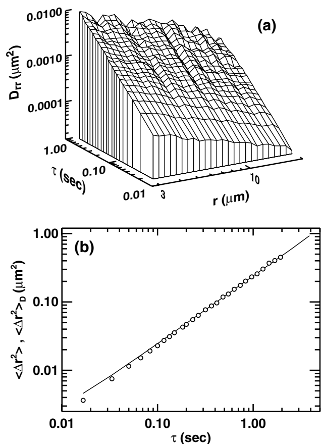
FIG. 1. (a) Two-point correlation function, D_{rr} , for 0.47 \mu\text{m} diameter beads dispersed in a glycerol/water solution, as a function of r and \tau . In a triple-log plot, the surface is a plane and is \propto \tau/r . (b) \langle \Delta r^2(\tau) \rangle_D calculated from D_{rr} (circles) overlaid on \langle \Delta r^2(\tau) \rangle (line). The agreement between the two indicates that the fluid satisfies Eq. (1).
