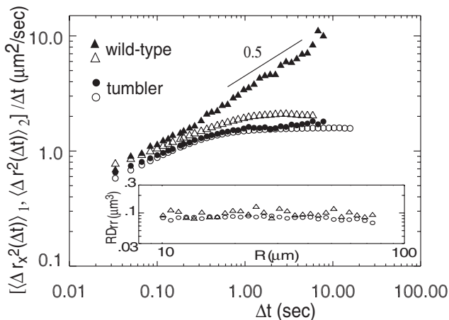
FIG. 1. 1-pt (open symbols) and 2-pt (closed symbols) mean-square displacements divided by the lag time, \Delta t , for 2a/\lambda = 2 \mu\text{m} particles in bath of wild-type RP437 (triangles) and tumbling RP1616 (circles) bacteria at \eta = 0.003 . Inset: D_{rr}(R, \Delta t) \sim 0.067 sec demonstrating D_{rr} \sim 1/R for R/\lambda = 10 , and implying correlation length \lambda \leq 10 \mu\text{m} .
