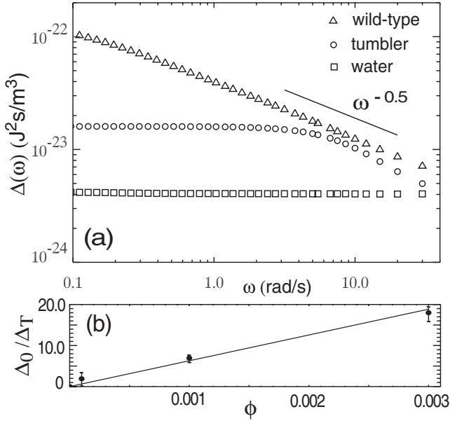
FIG. 4. (a) The spectrum \Delta \omega \psi of active stress fluctuations obtained from two-point microrheology and active response measurements. The triangles are the wild types, circles are the tumblers (both \phi = 0.003 ), squares are water ( \phi = 0 ). (b) Linear dependence of the prefactor \Delta_0 in \Delta \omega \psi on the volume fraction \phi of the wild-type bacteria; \Delta_{T\psi} = 2\eta k_B T .
