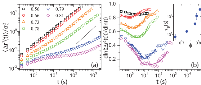
FIG. 1. (a) Log-log plot of the MSD, \langle r^2(t) \rangle , versus lag time t for different \phi . \langle r^2(t) \rangle is scaled by the square of the small sphere diameter, \sigma_s . The solid black line has unit slope. (b) Derivative of the logarithm of \langle r^2(t) \rangle with respect to logarithm of time, \frac{d \ln \langle r^2(t) \rangle}{d \ln(t)} , versus t at various \phi . The symbol and color code for \phi are the same as in (a). Solid colored lines are polynomial fits to the data near the minima. Inset shows variation of \tau_\beta with \phi . Note, the lack of clear minimum at \phi = 0.56 prevented estimation of its \tau_\beta .
