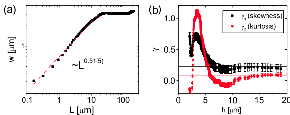
FIG. 3 (color online). (a) Width w plotted versus probed length scale L for a drop containing slightly anisotropic particles \varepsilon = 1.2 with height \bar{h} = 13 \mu\text{m} . The dashed line represents the best power-law fit for L < 15 \mu\text{m} . The observed power-law scaling is consistent with the KPZ universality class. (b) Skewness ( \gamma_1 ) and kurtosis ( \gamma_2 ) of the h distribution for particles with \varepsilon = 1.2 are plotted versus h . Solid lines represent values of \gamma_1 and \gamma_2 for Gaussian unitary ensemble matrices. Thus, the skewness and kurtosis imply that the height distribution is consistent with the KPZ universality class.
