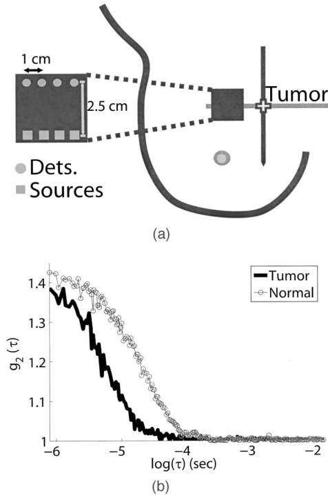
Fig. 1. (a) Hand-held probe with four source–detector pairs scanned horizontally and vertically in 1 cm increments spanning the estimated tumor region as well as the surrounding healthy tissue. (b) Temporal autocorrelation curves measured in the tumor (dark) and healthy (light) tissues of a patient. Faster decay corresponds to increased blood flow.
