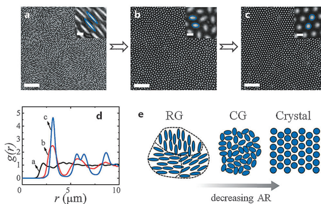
Figure 4. Shape transformations of an assembly of PS ellipsoids by a temperature trigger in a WL mixture ( C_L=0.2 ). a)–c) Bright-field micrographs. From (a) to (c), the ellipsoid aspect ratio AR is 4.4, 1.4, 1.0, respectively, with corresponding area fractions \phi=0.714 , 0.693, and 0.725, respectively. Insets: enlarged micrographs with blue curves to highlight the particle shape. d) Radial distribution function g(r) for panels a–c. e) Illustration of phases of the ellipsoid assemblies in two dimensions. As the aspect ratio decreases, the ellipsoids form a rotational glass (RG) with nematic domains, a conventional glass (CG) without nematic domains, and finally a crystal when AR \approx 1 . For panels (a)–(c), the scale bars are 20 \mu\text{m} (main figure) and 2 \mu\text{m} (inset).
