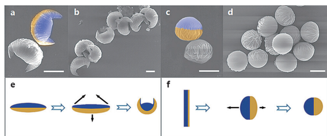
Figure 5. Fabrication of colloidal particles with novel shapes in a WL mixture ( C_L=0.2 ). Top panel: SEM images of the special PS colloidal particles: ox-horn-like (a, b) and Janus corrugated particles (c, d). Scale bar: 2 \mu\text{m} . Bottom panel: Particle fabrication. A thin layer of gold is coated onto one side of particle (yellow shading); then, during the shape recovery period, the different balances between the surface tension, elasticity of the metal coating, and viscosity of the particle interior produce uniquely shaped particles. The solid black arrows indicate the force directions, and the lengths of the arrows indicate the force magnitudes.
