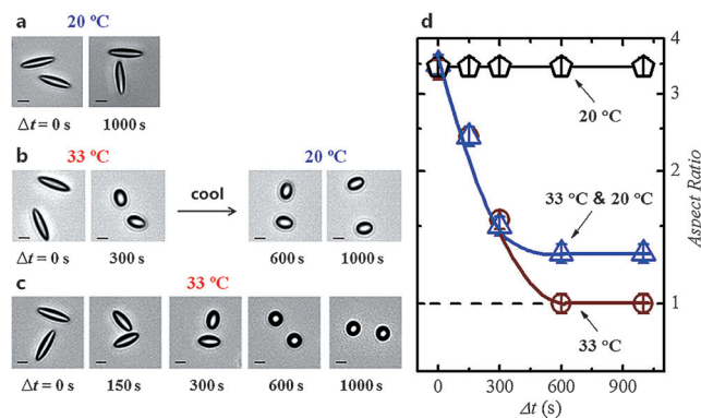
Figure 2. Bright-field micrographs of the stimuli-responsive shape transformation of PS ellipsoids in a water/2,6-lutidine mixture ( C_L=0.2 ). a) At 20 °C, PS ellipsoids maintain their shape. b) Heating the system to 33 °C activates the shape-switching of the PS ellipsoids; cooling the system stops the transformation, and the new shape is preserved. c) Without cooling, particles transform continuously from ellipsoids to spheres. d) The corresponding aspect ratios ( AR = \text{long axis}/\text{short axis} ) of the particles are shown in a, b, and c. Scale bar: 2 \mu\text{m} . See the Supporting Information Movies S1 and S2 for the videos of the shape transformations in (b) and (c).
