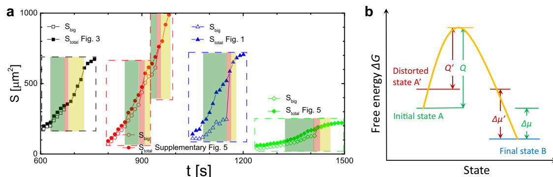
Fig. 6 | Crystal growth during nucleus coalescence. a The evolution of the nucleus area S for the larger nucleus (open symbols, S_{\text{big}} ) and for the sum of two nuclei (solid symbols, S_{\text{total}} ) for Fig. 3 (black square), Supplementary Fig. 5 (red circle for two coalescence events), Fig. 1 (blue triangle), and Fig. 5 (green diamond). The
