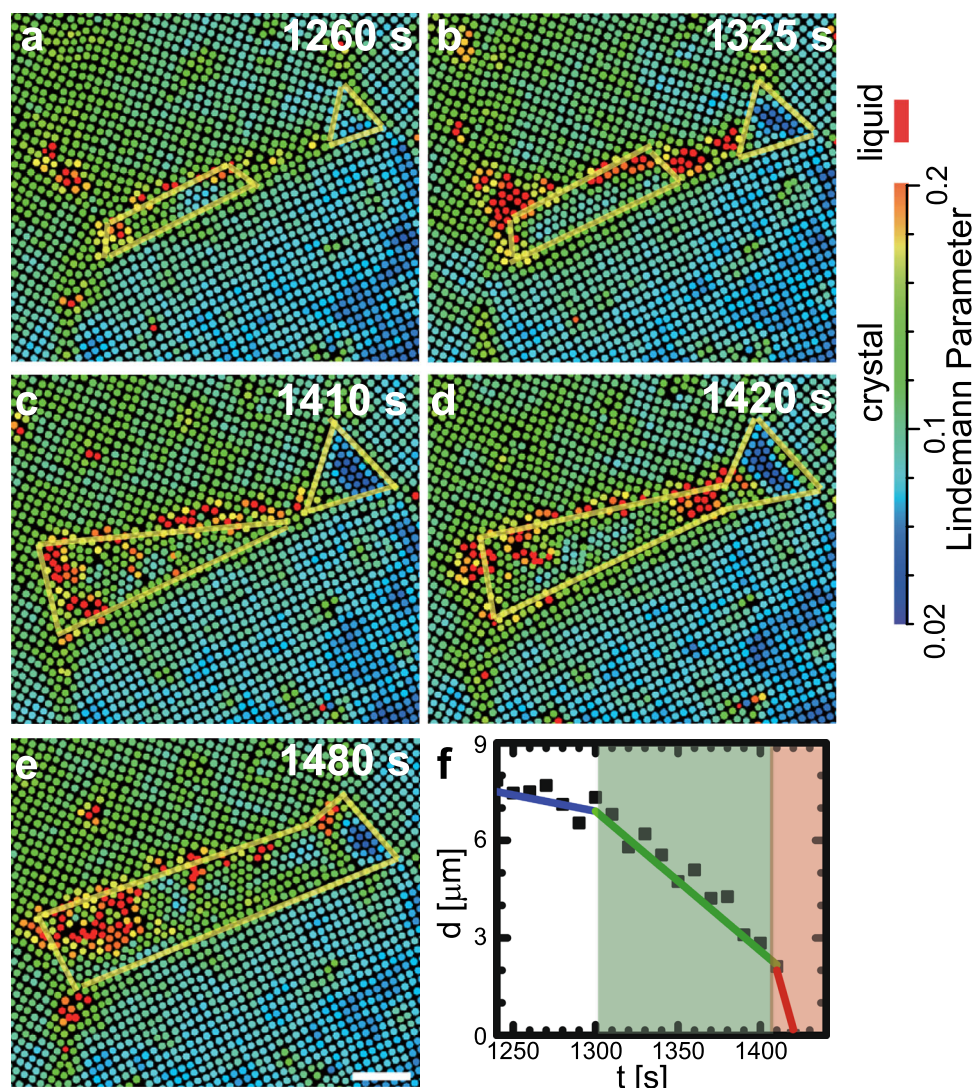
Fig. 5 | Coalescence of nuclei on a high-angle (45°) GB. a At t = 1260 s, notice a rectangular nucleus on a GB and a triangular nucleus at a triple junction. b At t = 1325 s, both nuclei grow. c The nucleus on the GB grows towards the triple junction and becomes triangular in shape. d Two nuclei merge together. e The
