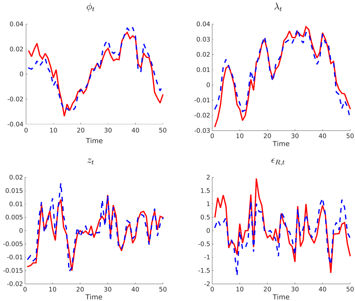
Figure 25: Particle-Filtered States
