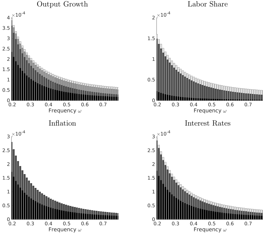
Figure 18: Spectral Decomposition
