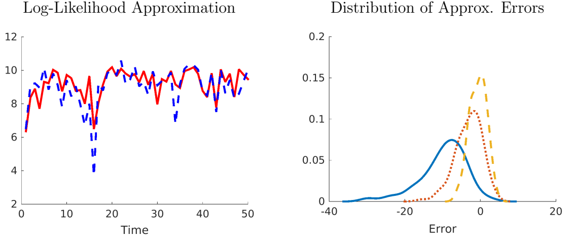
Figure 26: Particle-Filtered Log-Likelihood
