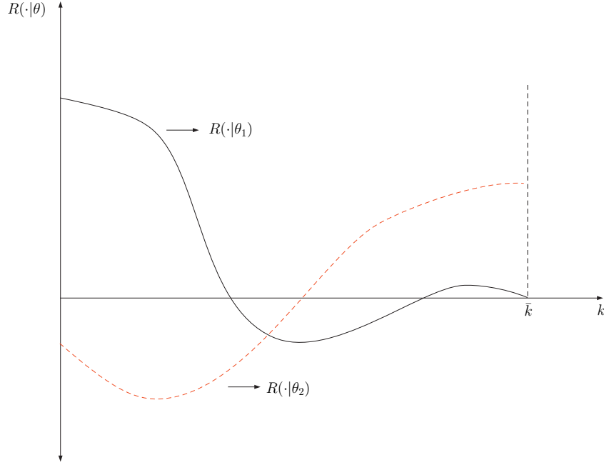
Figure 2: Residual Functions
