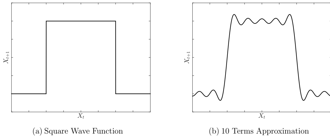
Figure 4: Gibbs Phenomenon
