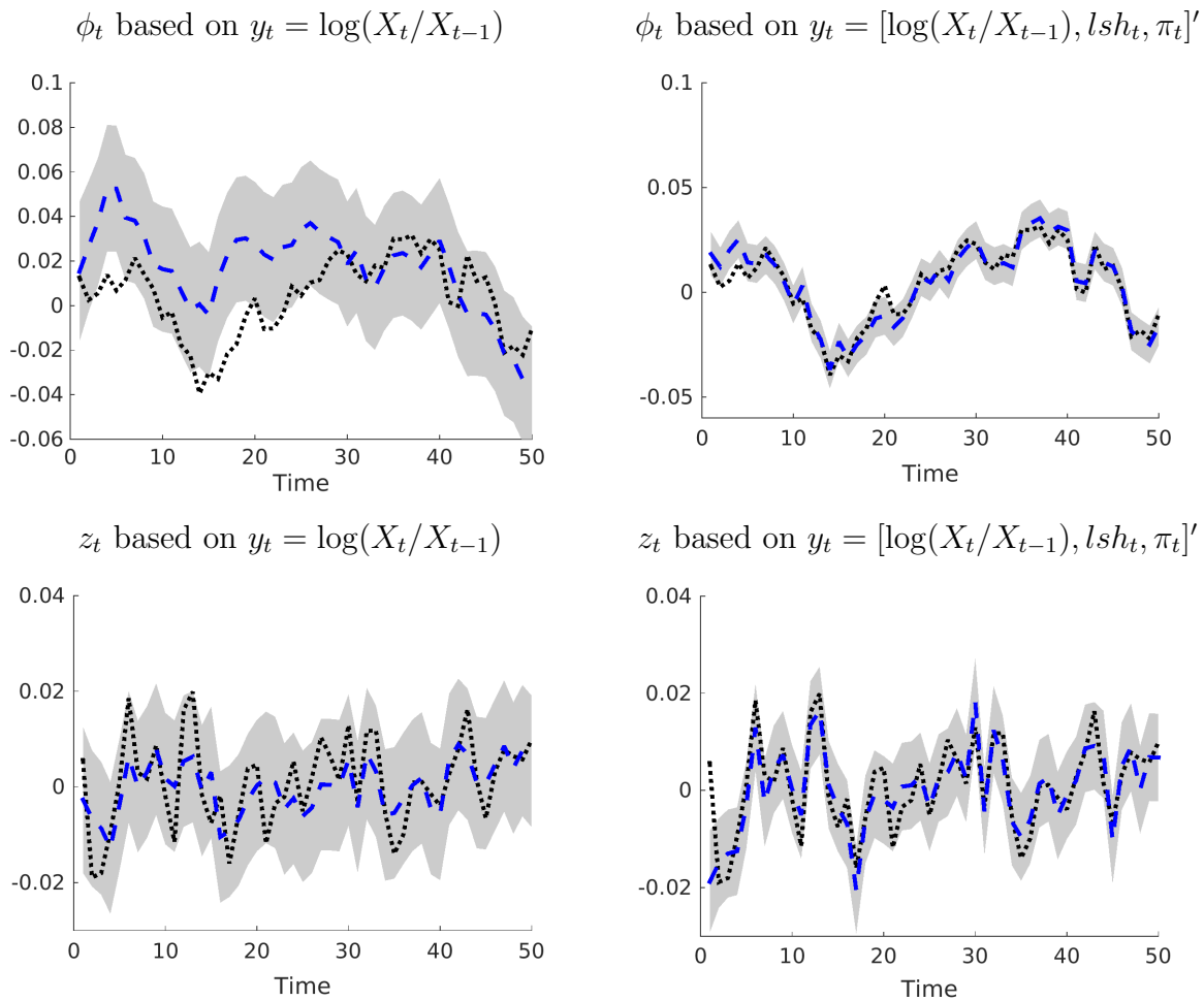
Figure 24: Filtered States
