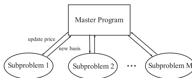
Fig. 4. Interactions in DW decomposition.
