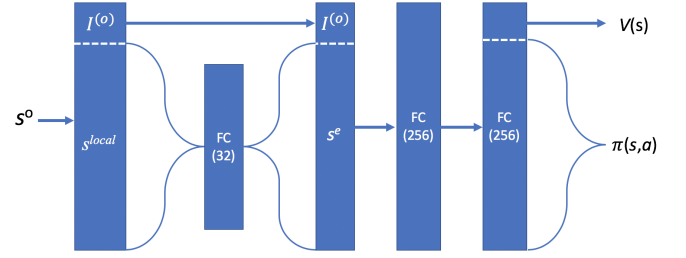
Fig. 3. Illustration of the neural network architecture for A2C with shared layers between the actor and critic. Each hidden layer is a fully connected (FC) layer with 32 nodes for the encoded state and 256 nodes for the last two layers.
