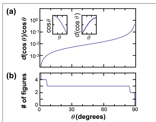
Fig. 2. Determination of the number of significant figures for the cosine function using error analysis. (a) The normalized uncertainty for the cosine function plotted against the input angle. All input angles are assumed to be precise to the one's place and have an uncertainty of 0.5^\circ . Inset, graph of the cosine function and the uncertainty in the cosine function versus angle in degrees (from 0^\circ to 90^\circ ). (b) The number of significant figures for the cosine function versus input angle. For a complete discussion see the online appendix. 33
